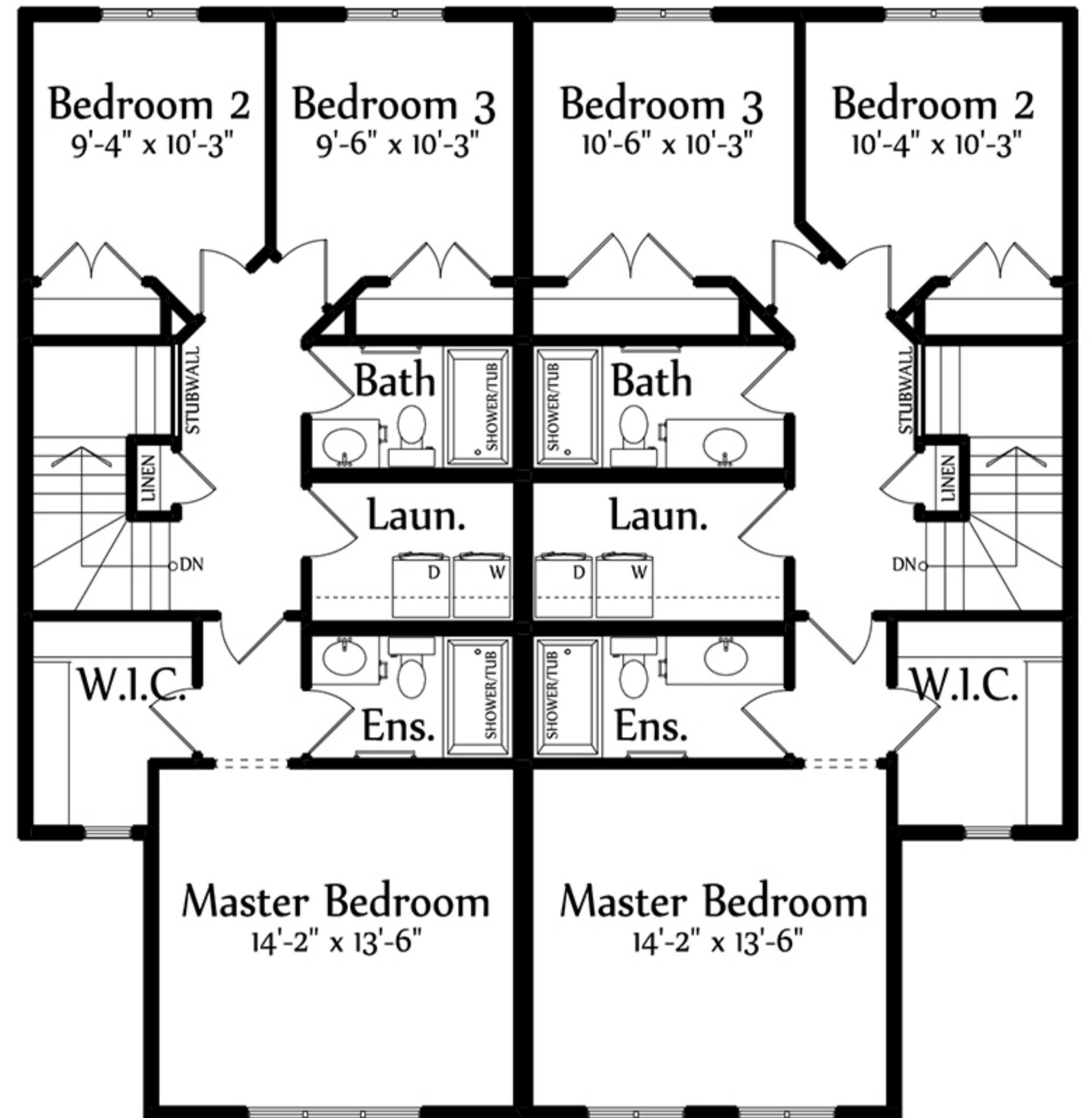
SECOND FLOOR PLAN 769/835 Sq.Ft.
