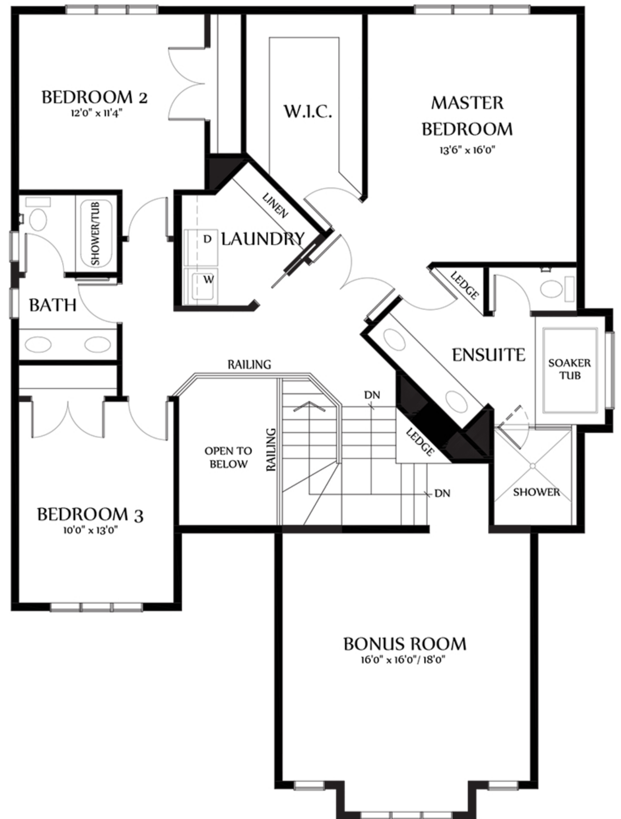
SECOND FLOOR PLAN 1,503 Sq.Ft.
