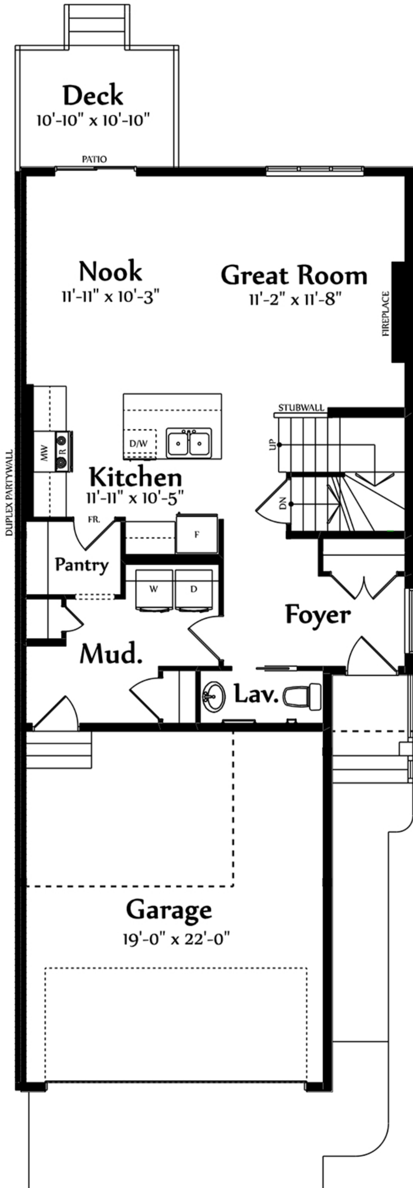
MAIN FLOOR PLAN 750 Sq.Ft.
