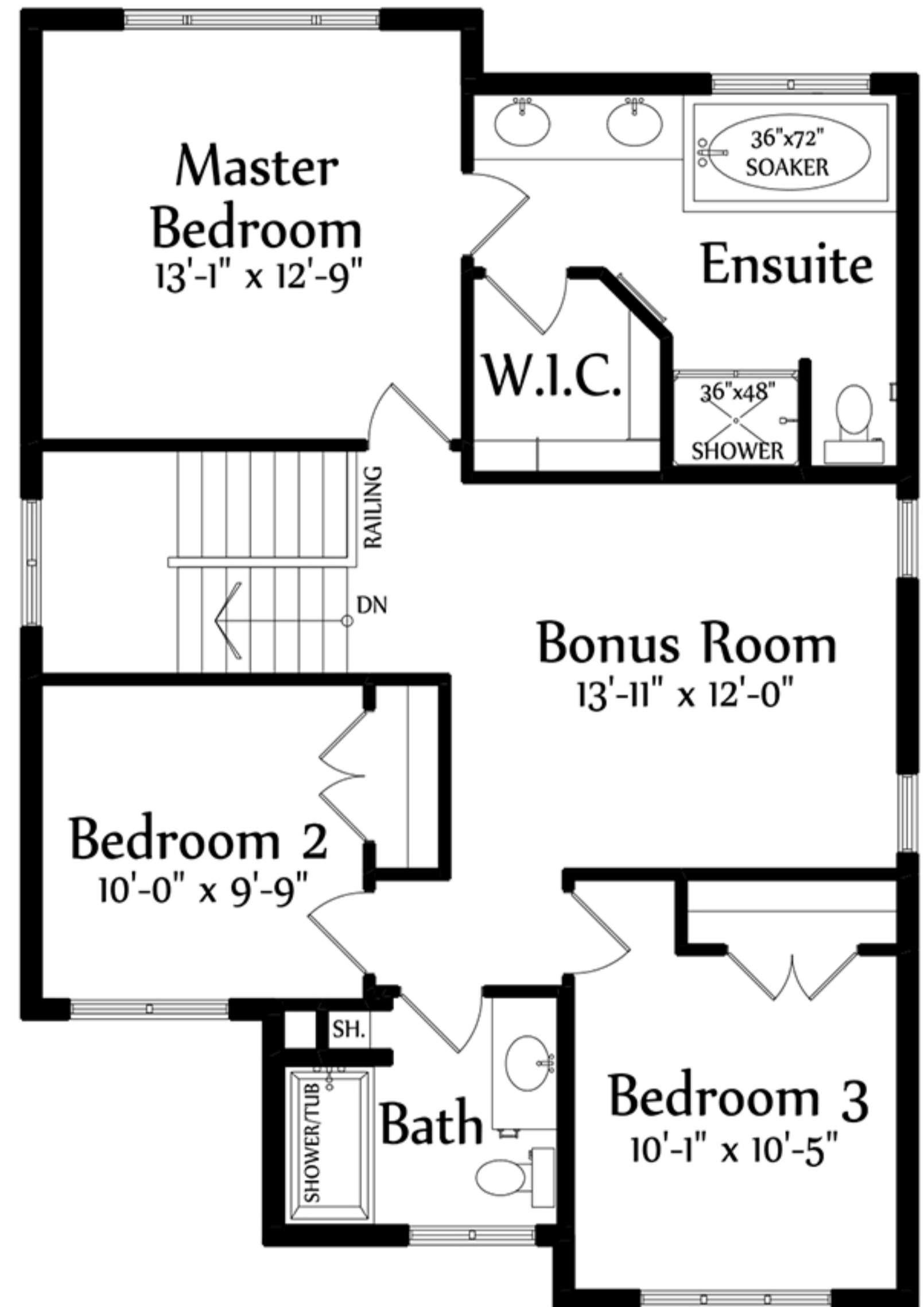
SECOND FLOOR PLAN 919 Sq.Ft.
