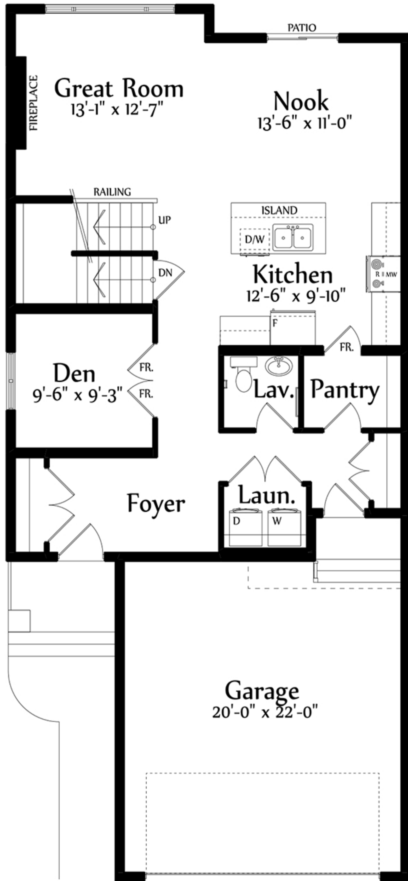
MAIN FLOOR PLAN 1,009 Sq.Ft.
