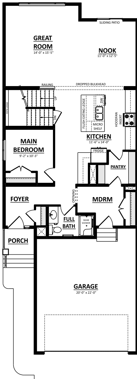
MAIN FLOOR PLAN (OPT. BED & FULL BATH) 1109 Sq.Ft.
