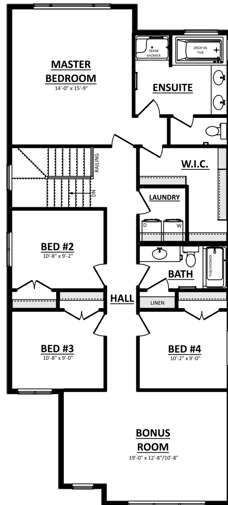
SECOND FLOOR PLAN (OPT. FRONT BONUS) 1323 Sq.Ft.
