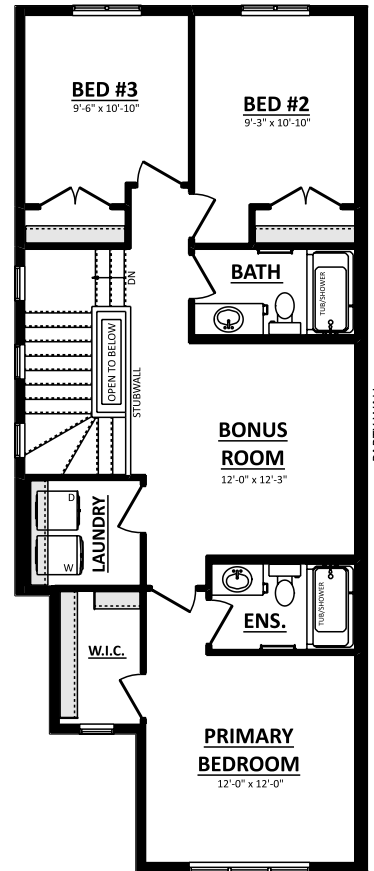
SECOND FLOOR PLAN 845 Sq.Ft.
