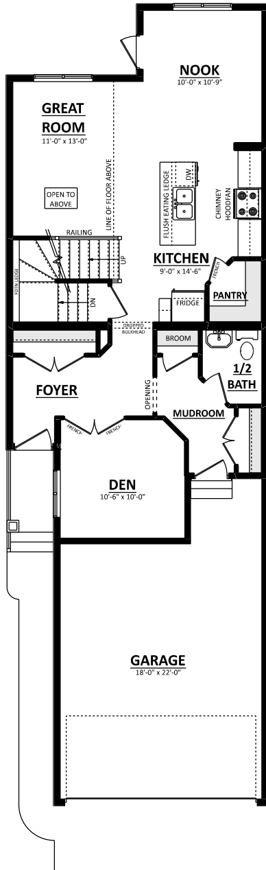
MAIN FLOOR PLAN (OPTIONAL DEN) 867 Sq.Ft.
