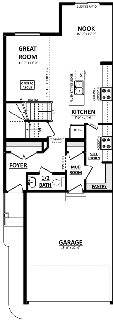
MAIN FLOOR PLAN (OPT. SPICE KITCHEN) 759 Sq.Ft.
