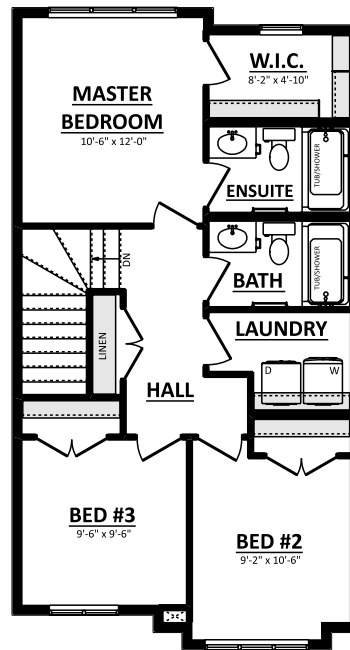
SECOND FLOOR PLAN 669 Sq.Ft.
