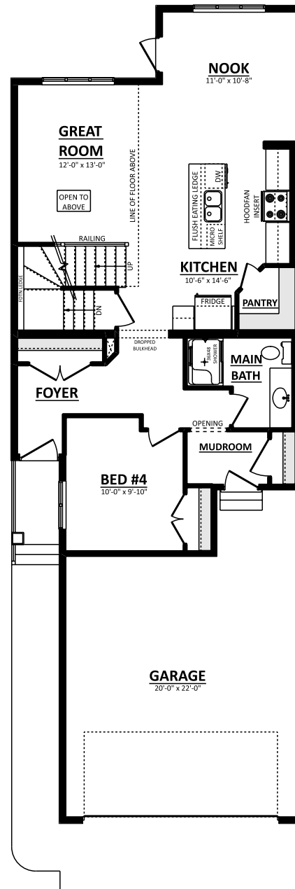
MAIN FLOOR PLAN (OPT. BED & BATH) 950 Sq.Ft.
