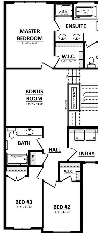
SECOND FLOOR PLAN *Opt. Reversed Stairs* 1006 Sq.Ft.
