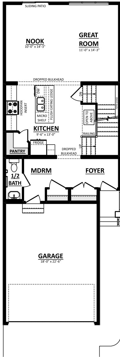
MAIN FLOOR PLAN *Opt. Reversed Stairs* 815 Sq.Ft.
