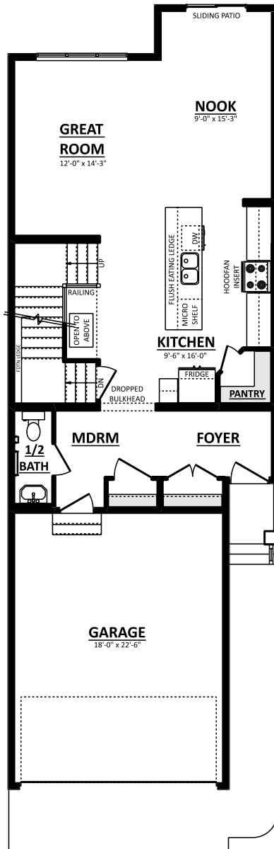
MAIN FLOOR PLAN (OPT. NOOK/KITCHEN) 855 Sq.Ft.
