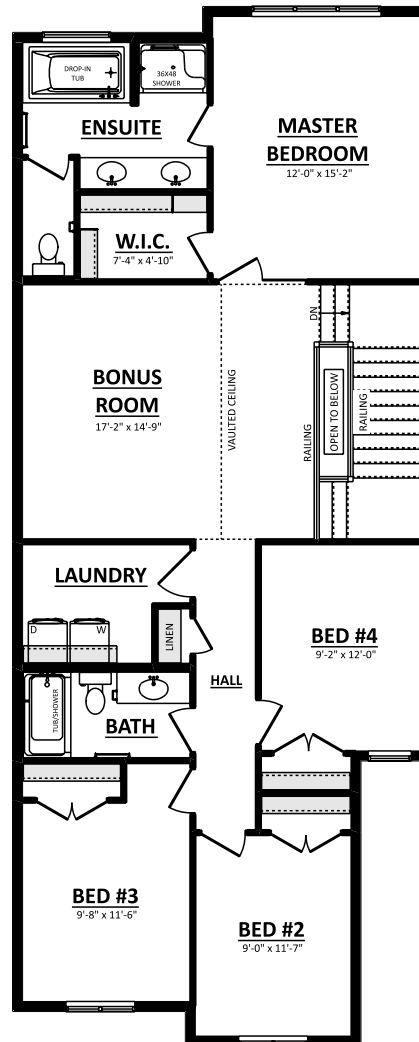
SECOND FLOOR PLAN (OPT. 4TH BEDROOM) 1252 Sq.Ft.
