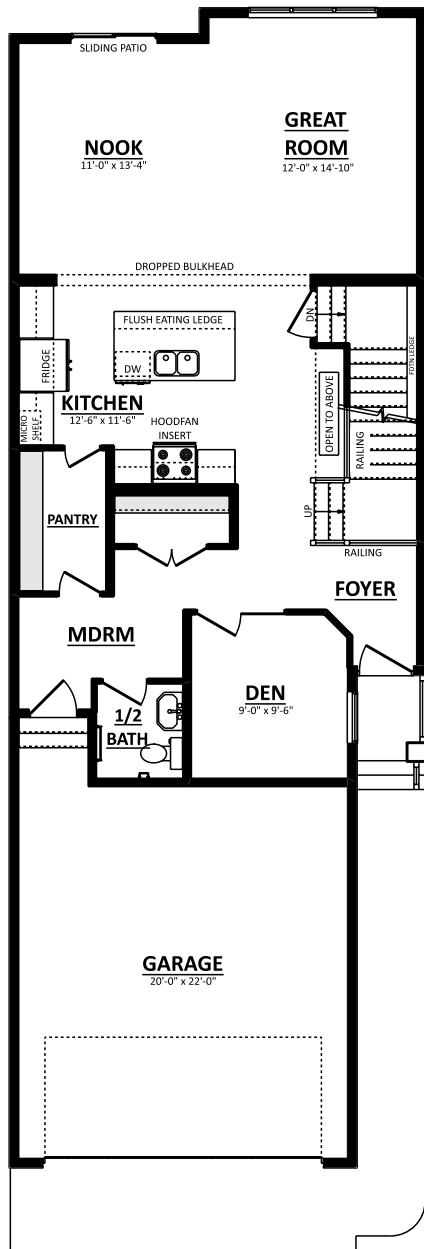
MAIN FLOOR PLAN (OPTIONAL DEN) 1020 Sq.Ft.
