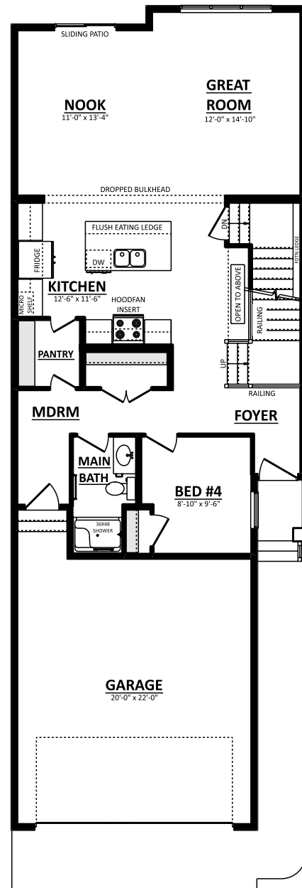
MAIN FLOOR PLAN (OPT. BED & BATH) 1020 Sq.Ft.
