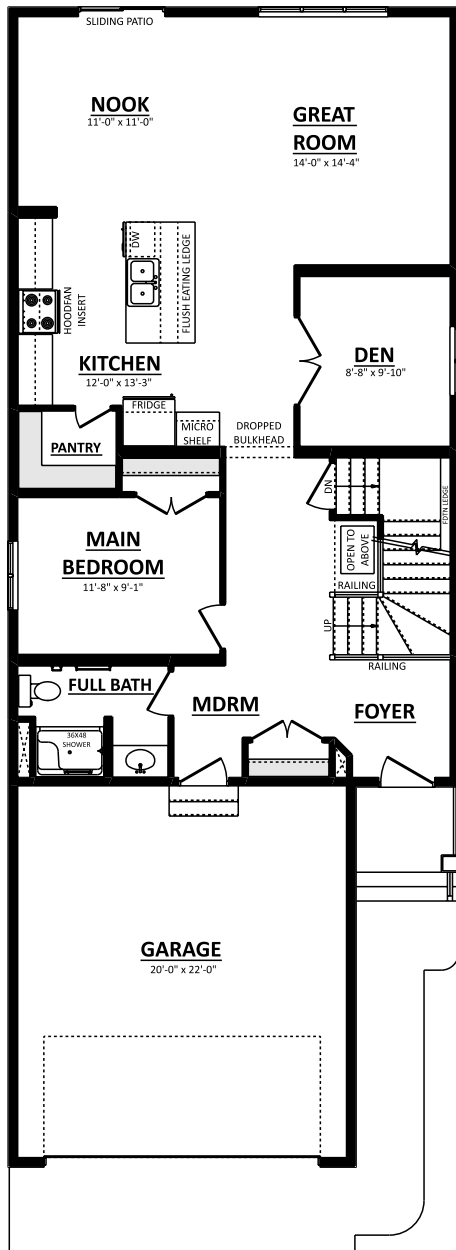
MAIN FLOOR PLAN (OPT. BED & FULL BATH) 1170 Sq.Ft.
