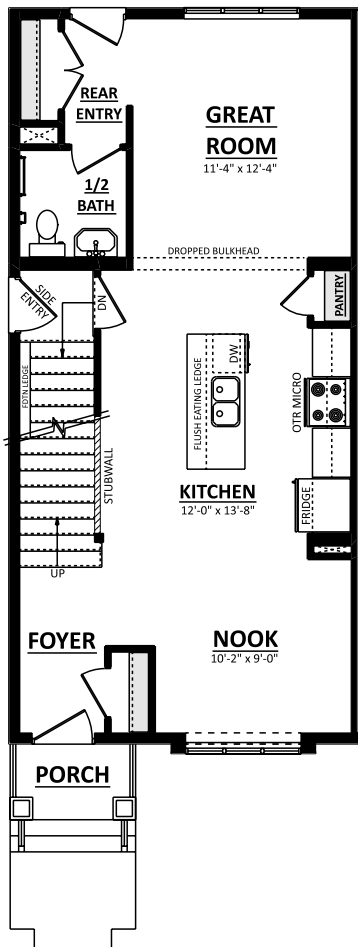
MAIN FLOOR PLAN 684 Sq.Ft.
