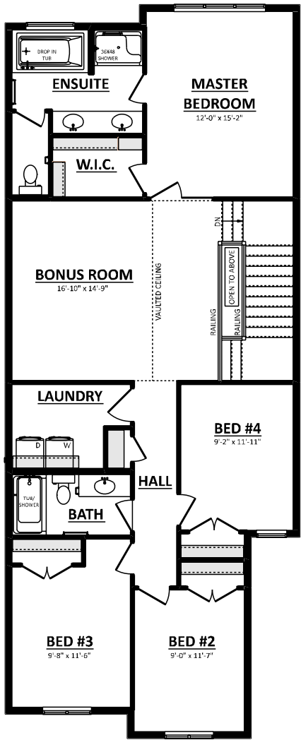
SECOND FLOOR PLAN 1252 Sq.Ft.
