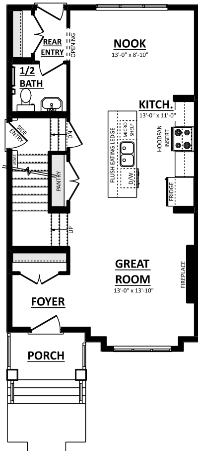
MAIN FLOOR PLAN 700 Sq.Ft.
