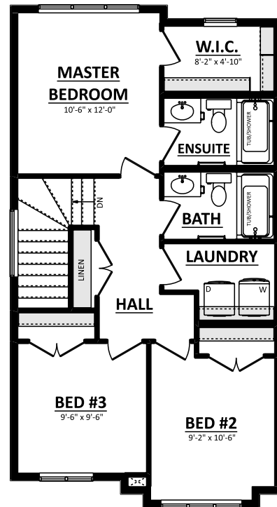
SECOND FLOOR PLAN 669 Sq.Ft.
