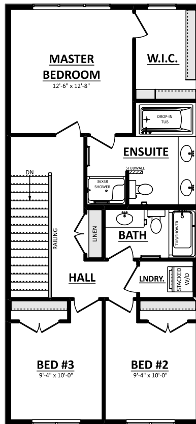
SECOND FLOOR PLAN (OPT. ENSUITE) 805 Sq.Ft.
