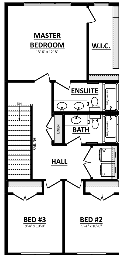
SECOND FLOOR PLAN 805 Sq.Ft.
