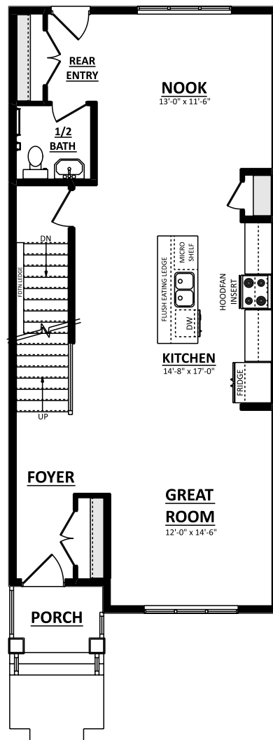
MAIN FLOOR PLAN (OPT. CENTER KITCHEN) 886 Sq.Ft.
