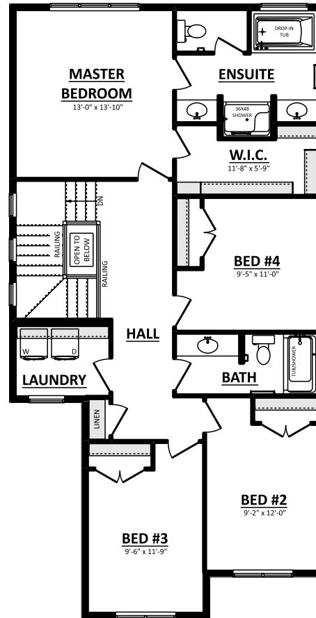
SECOND FLOOR PLAN (OPT. 4TH BEDROOM) 1103 Sq.Ft.
