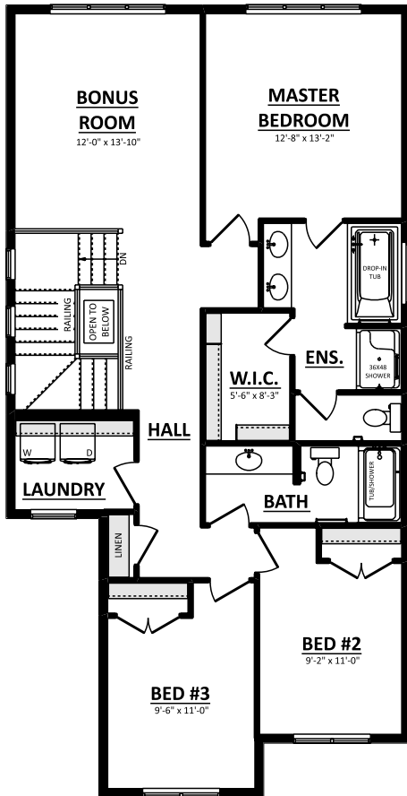
SECOND FLOOR PLAN (OPT. REAR BONUS) 1103 Sq.Ft.
