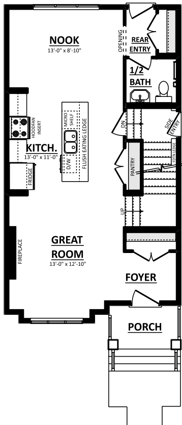
MAIN FLOOR PLAN 700 Sq.Ft.
