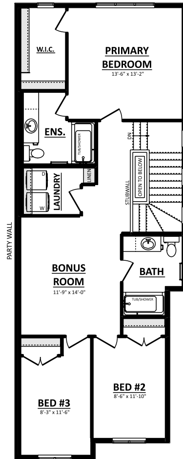
SECOND FLOOR PLAN (Opt. Layout) 940 Sq.Ft.
