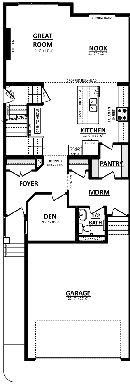
MAIN FLOOR PLAN (Opt. Den) 1016 Sq.Ft.
