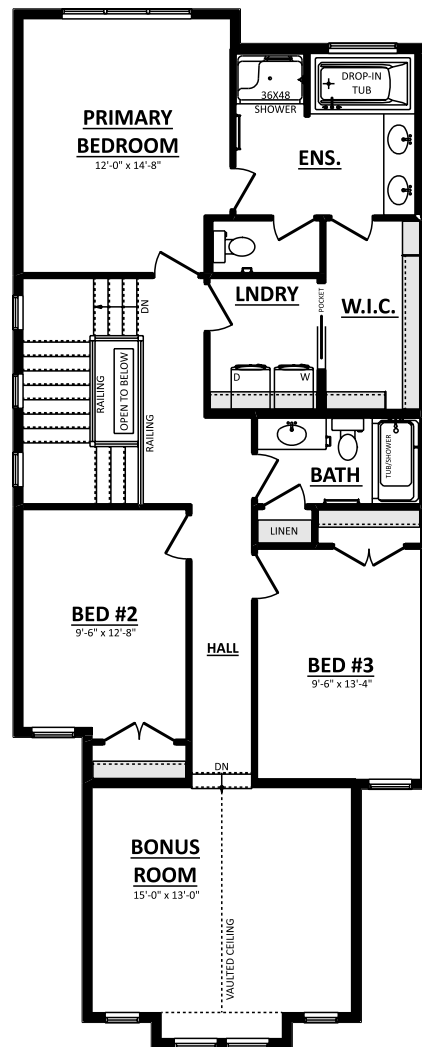
SECOND FLOOR PLAN (Opt. Dropped Bonus) 1180 Sq.Ft.
