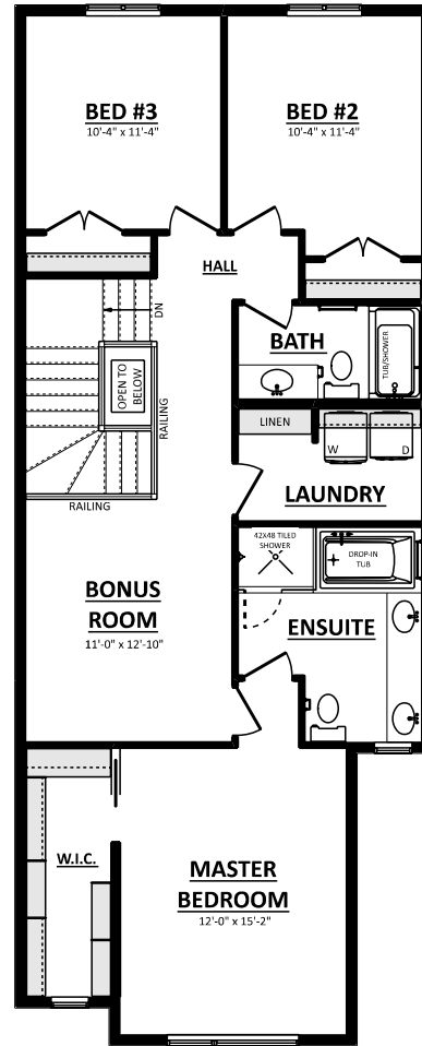
SECOND FLOOR PLAN 1056 Sq.Ft.
