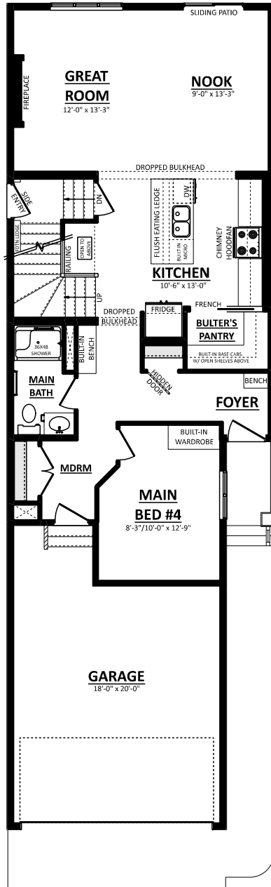
MAIN FLOOR PLAN (OPT. BED & BATH) 973 Sq.Ft.
